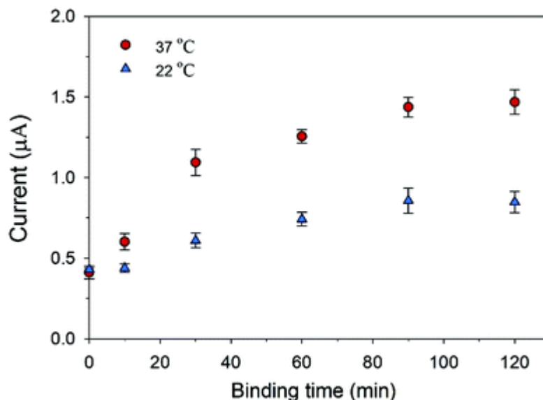
Fig. 3 Optimization of the binding condition of GBPs-ALP onto the gold electrode. Dependence of the electrochemical signal on increased binding time (0, 10, 30, 60, 90, and 120 min) at 37 °C (red circle) and 22 °C (blue triangle), respectively. Error bars represent standard deviation of six independent replicates.
